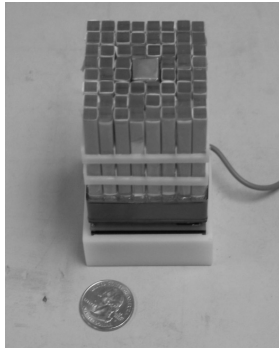
FIGURE 1. GRAPE Science Model 3 (SM3) fully populated with 60 plastic scintillators and a central CsI(Na) calorimeter.
