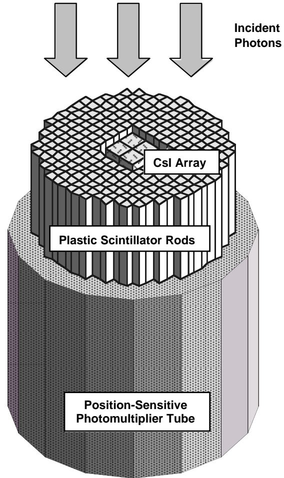
Figure 4: The SOLPOL polarimeter design showing the layout of the plastic scintillator elements and CsI(Tl) elements on the front surface of a PSPMT. Not shown here is the 4-element multianode PMT used for readout of the CsI(Tl) array and the lead shield that would be used to block direct flux from the CsI(Tl) array.
