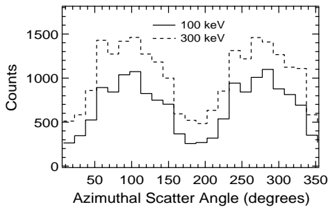
FIGURE 4. Simulated modulation curves (counts versus azimuthal scatter angle) at energies of 100 and 300 keV.
