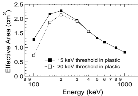
FIGURE 5. Effective area versus energy.
