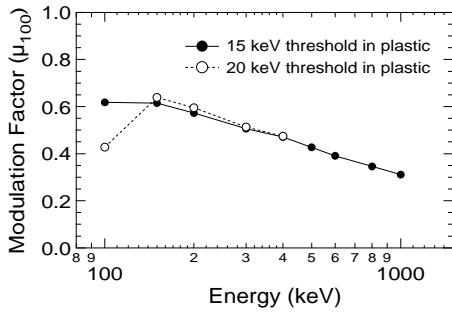
FIGURE 6. Modulation factor versus energy.
